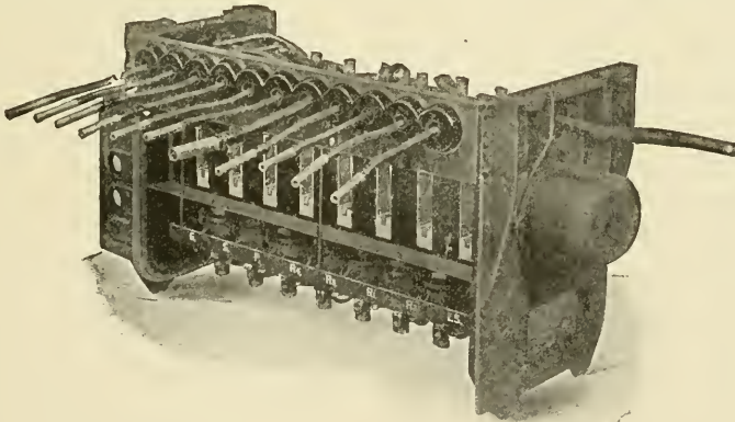
Fig. 71. Group of Unit Switches, Westinghouse System
